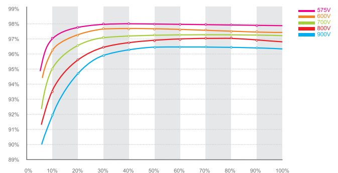
Growatt 9000UE efficiency
